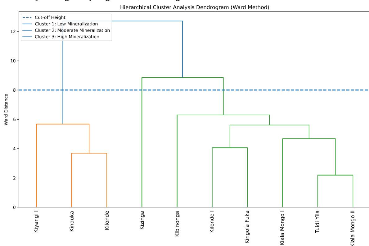
Figure 3. Dendrogram classification for different water sources
