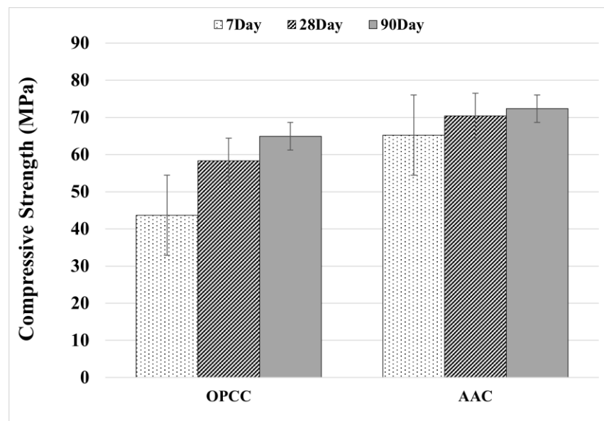
Figure 2. Compressive Strength Test Results
