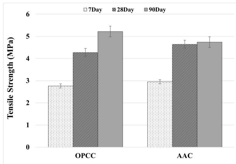
Figure 3. Tensile Strength Test Results
