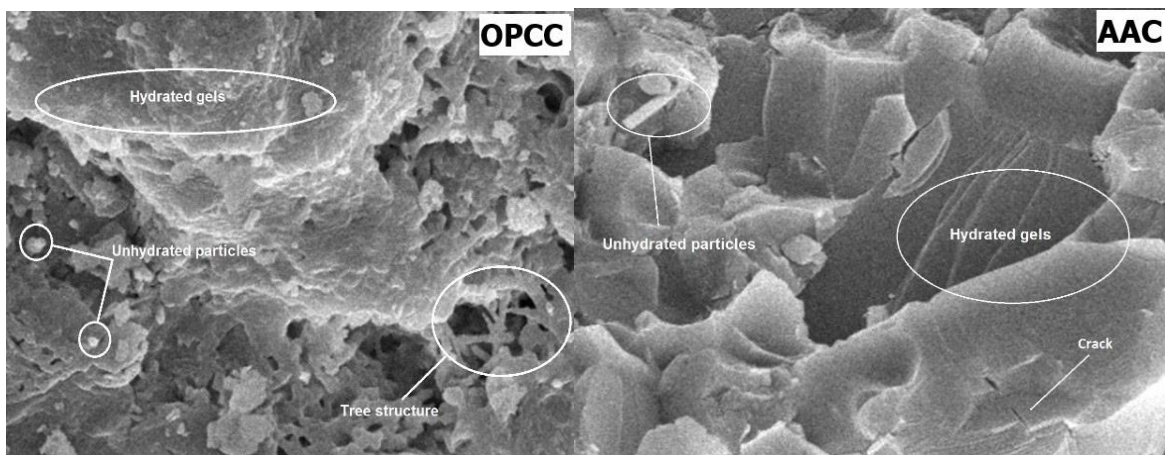
Figure 7. SEM Analysis Results
