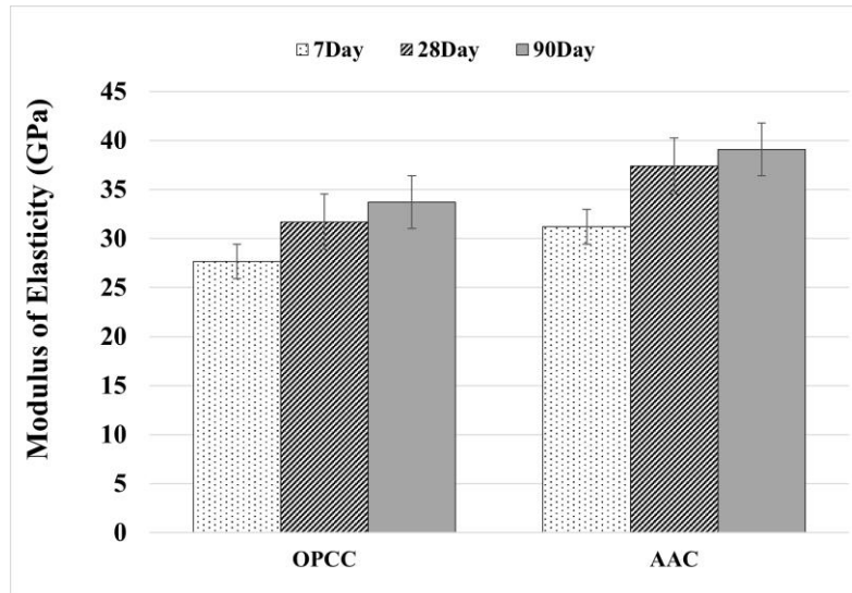
Figure 6. Results of the Modulus of Elasticity Test
