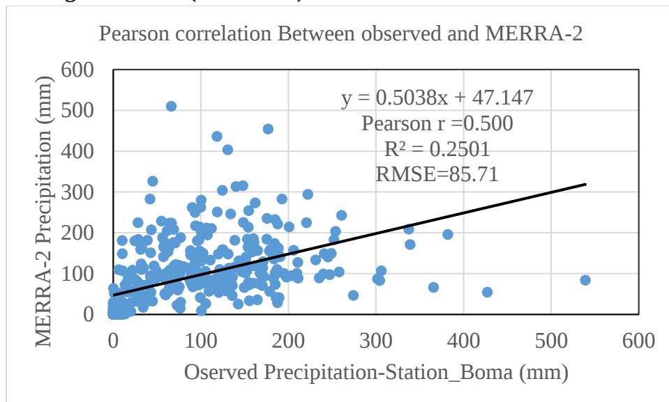
a) Linear regression and Pearson correlation analysis between observed monthly precipitation at Boma Meteorological Station and MERRA-2 reanalysis estimates
