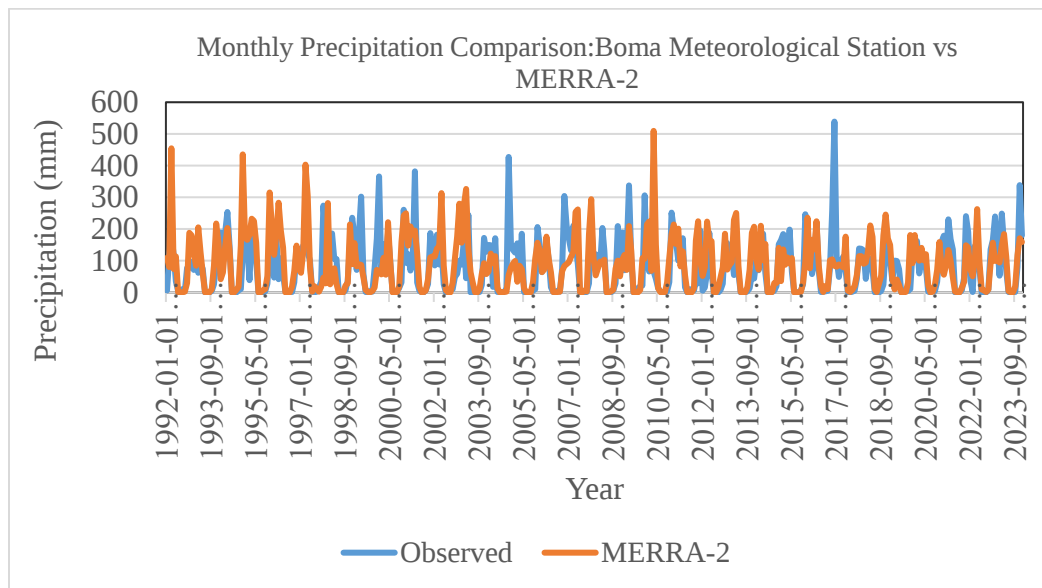
a) Comparative analysis of monthly precipitation time series derived from ground observations and MERRA-2 reanalysis data
