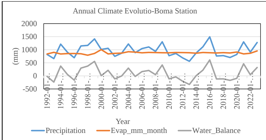
a) Annual evolution of climate variables (precipitation, evaporation, and water balance) at Boma station
