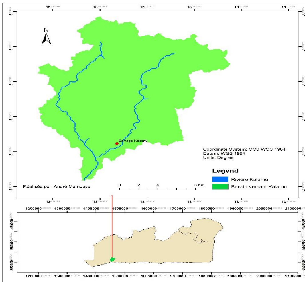
Figure 1. Kalamu River watershed at Boma
