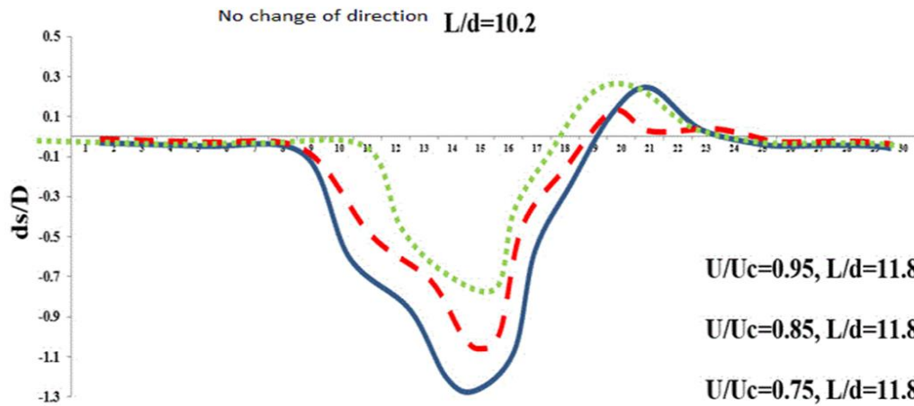
Figure 10. Effect of Relative Velocity and Channel Geometry on Scour Depth Profile ( ds/D ) at Various Flow Ratios ( U/U_c ).
