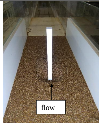
Figure 3. The base of the door change section L/d=13.4.
