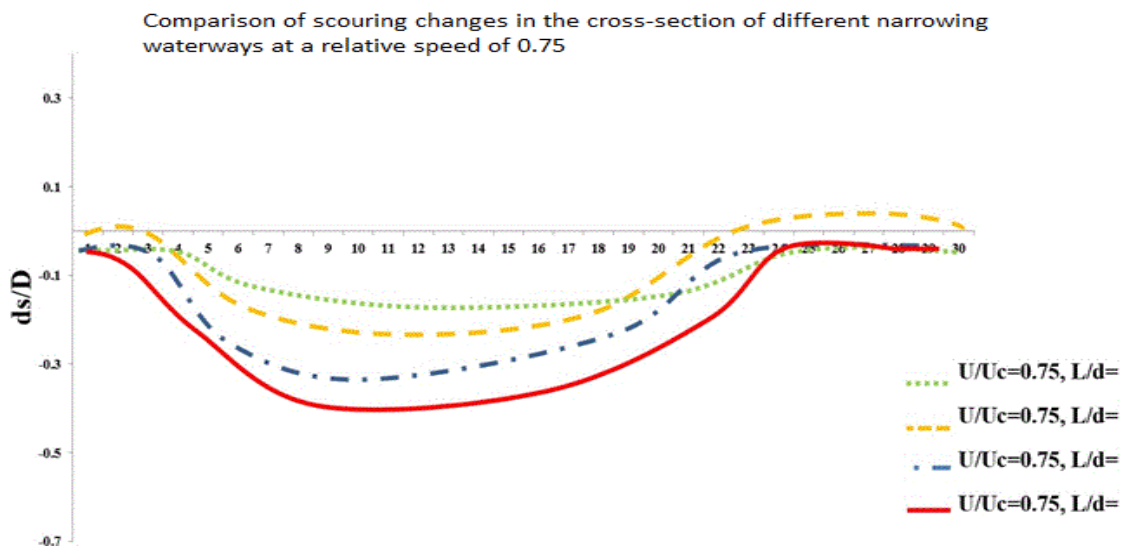
Figure 11. Comparison between the amount of scouring in different modified stages ( L/d=10.2, 11.8, 13.4, 15 ) at a relative speed of 0.75.
