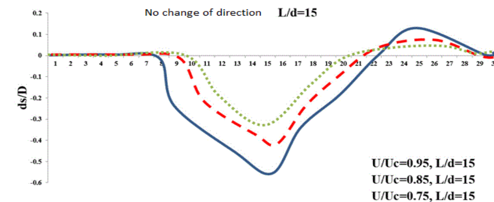
Figure 7. Comparison between the amount of scouring of the base in the case of no sudden change in the section of the waterway in relative velocities ( U/U_c=0.75, 0.85, 0.95 ).
