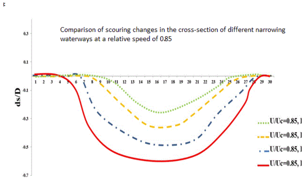
Figure 12. Comparison between the amount of scouring in different changed sections ( L/d=10.2, 11.8, 13.4, 15 ) at a relative speed of 0.85.
