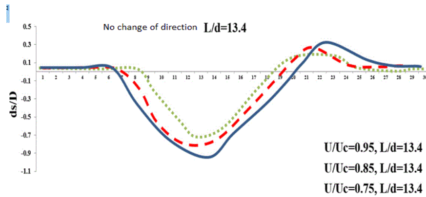
Figure 8. Comparison between the scour rate of the base in the state L/d=13.4 at relative velocities ( U/U_c=0.75, 0.85, 0.95 ).
