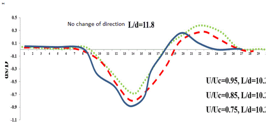
Figure 9. Comparison between the amount of scouring of the base in the state L/d=11.8 at relative velocities ( U/U_c=0.75, 0.85, 0.95 ).
