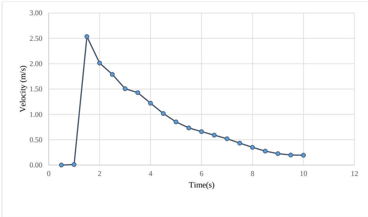
Figure 21. Velocity at Sensor 2 for the check dam with an opening width equal to 0.25 times the channel width.
