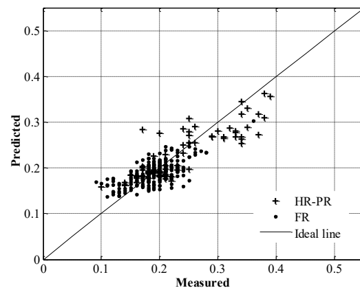
Figure 11. Comparison between the Andersen measured wave reflection coefficient and predicted values by the M5' MT algorithm
