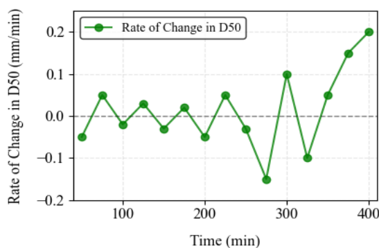
Figure 7. Rate of Change in Mean Grain Size ( d_{50} ) Over Time.
