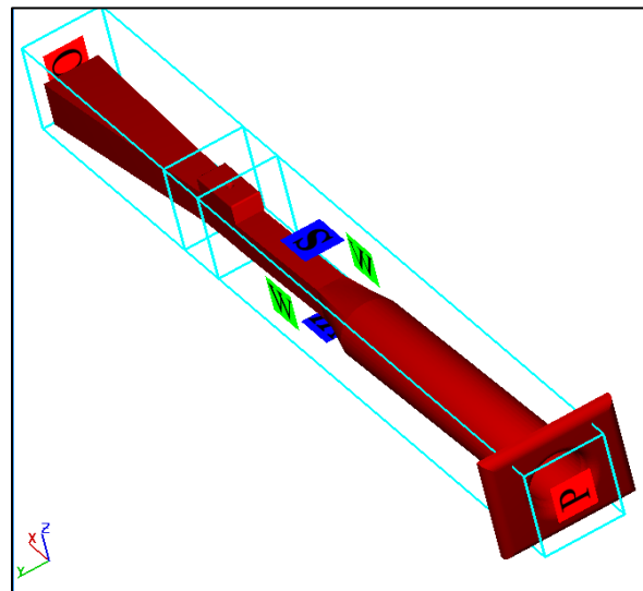
Figure 4. boundary condition in the numerical model.
