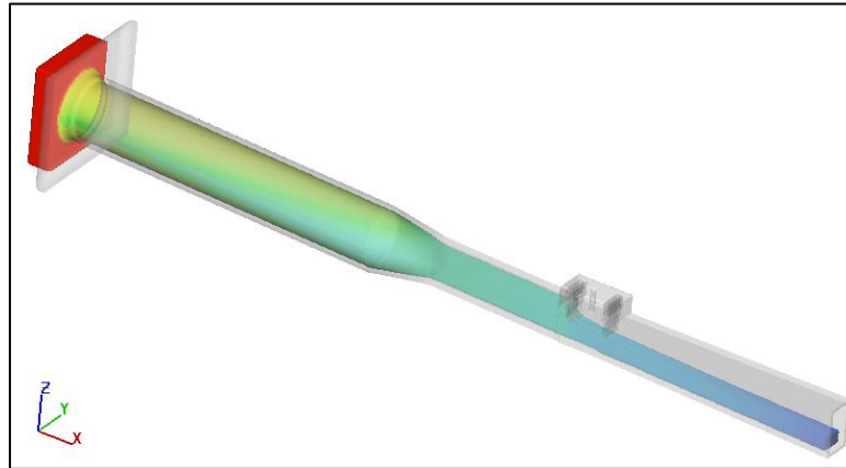
Figure 5. 3D hydrodynamic simulation of flow in the Siazakh Dam bottom outlet system with a 50% gate opening.
