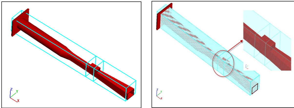
Figure 3(a) and (b). Mesh block of the Siazakh Dam's bottom outlet in the Flow-3D numerical model, along with computational cells on the mesh block in the Flow-3D model.
