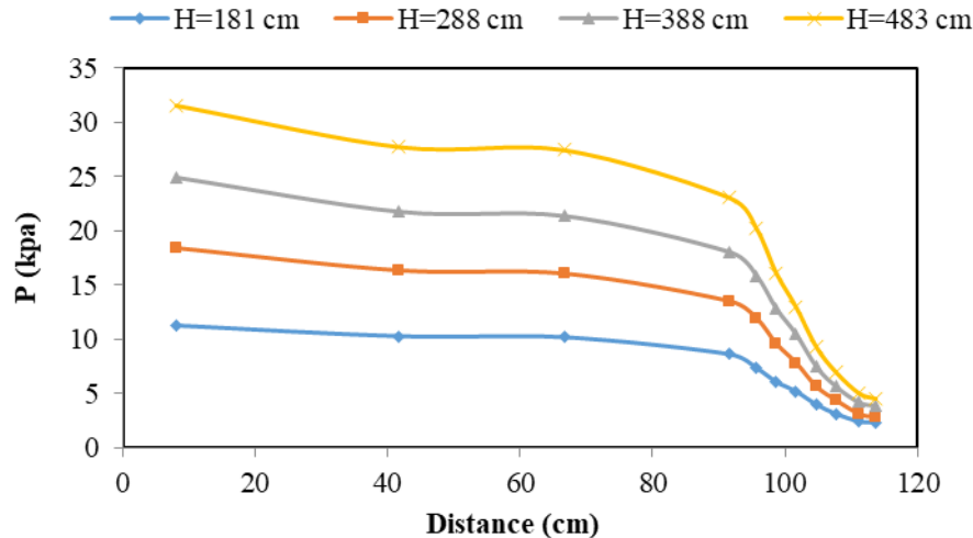
Figure 2. The pressure variations on the floor for a 100% gate opening.
