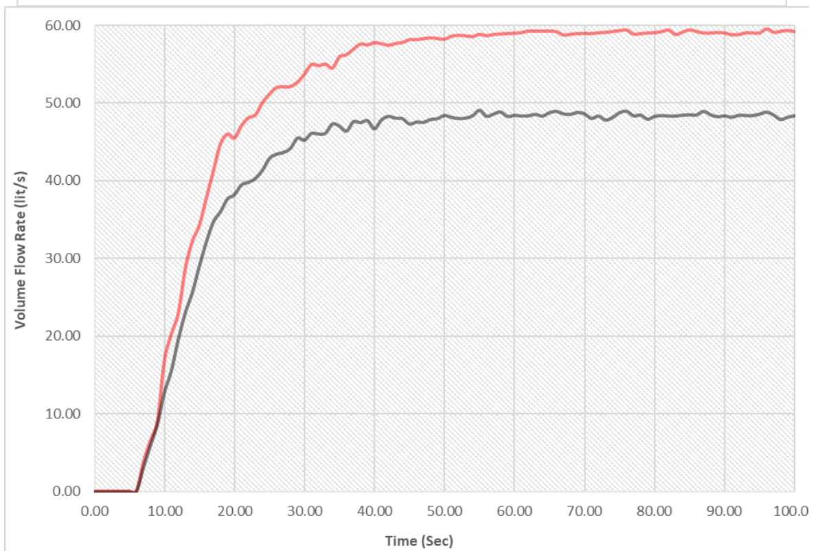
Figure 6 (a), (b), (c) and (d). (Continued) Outflow rate over time for sediment concentrations of 3000, 6000, 9000, and 12000 ppm.
