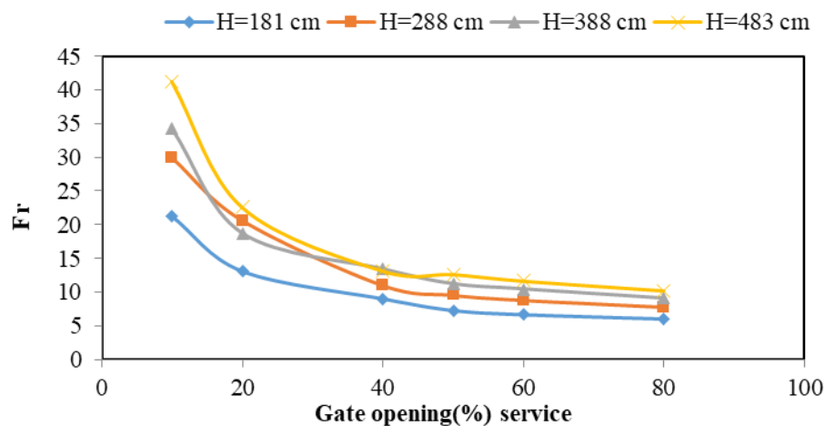
Figure 1. Changes in the Froude number within the discharge channel of the bottom outlet system.
