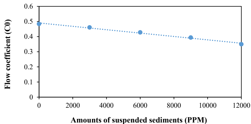
Figure 7. Variation of discharge coefficients with suspended load concentrations from 0 to 12000 ppm, illustrating the fitted relationship based on existing data.
