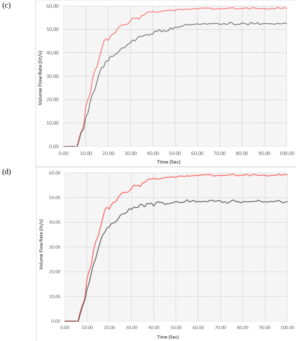
Figure 6 (a), (b), (c) and (d). (Continued) Outflow rate over time for sediment concentrations of 3000, 6000, 9000, and 12000 ppm.
