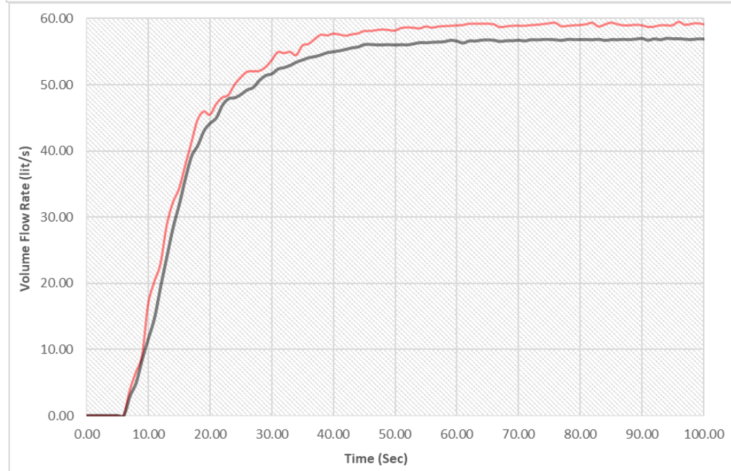
Figure 6 (a), (b), (c) and (d). Outflow rate over time for sediment concentrations of 3000, 6000, 9000, and 12000 ppm.
