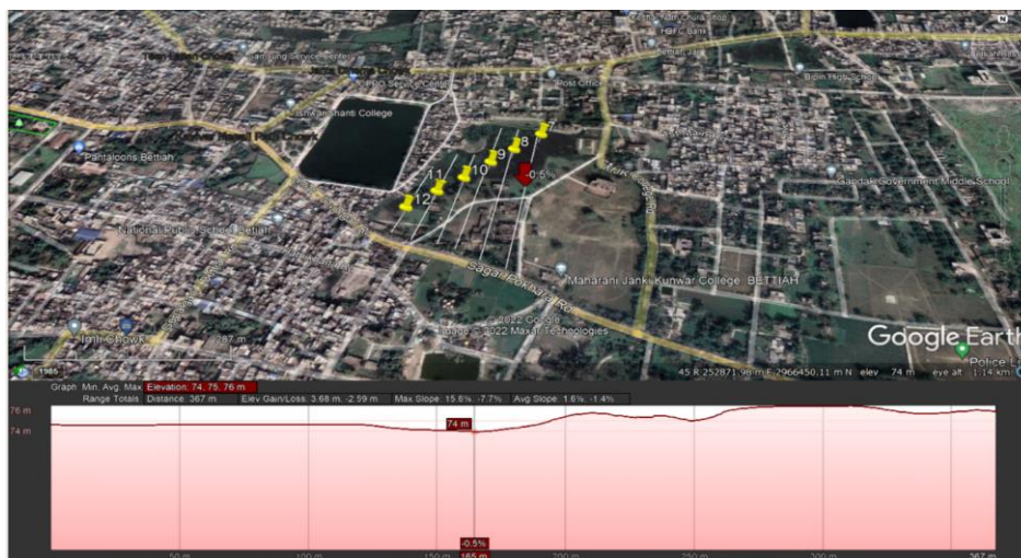
Figure 7. Elevation Profile of Line 6.
