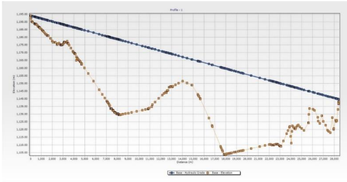
Figure 13. The hydraulic profile of the transmission line in a stable state (from the Kavardreh tank to the F zone tank)
