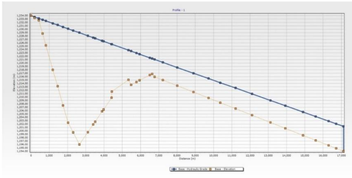
Figure 4. Hydraulic profile of transmission line in steady state (from Islamabad reservoir to Kavardeh reservoir)
