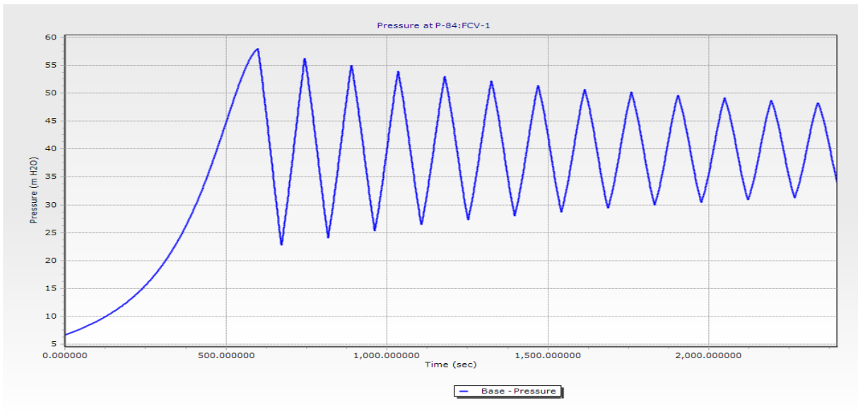
Figure 9. Pressure wave changes at the end of the path in case of controlled closing of the valve at the end of the path (from Islamabad tank to Kavardah tank)
