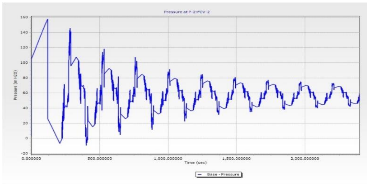
Figure 14. Pressure wave changes at the end of the path in case of sudden closing of the valve at the end of the path (from Kavardah tank to F zone tank)
