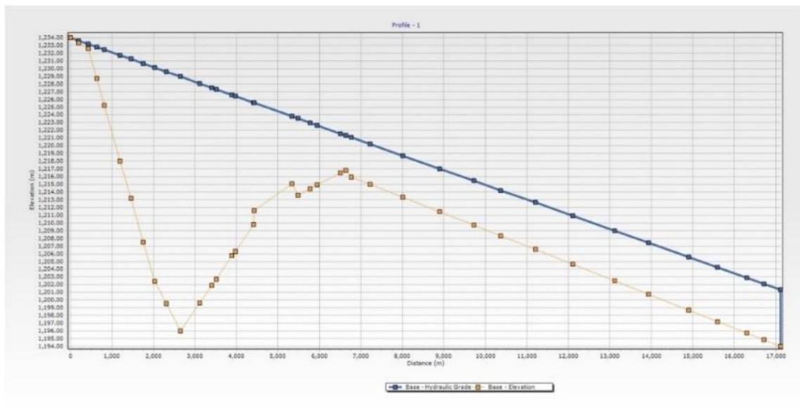
Figure 4. Hydraulic profile of transmission line in steady state (from Islamabad reservoir to Kavardreh reservoir)
