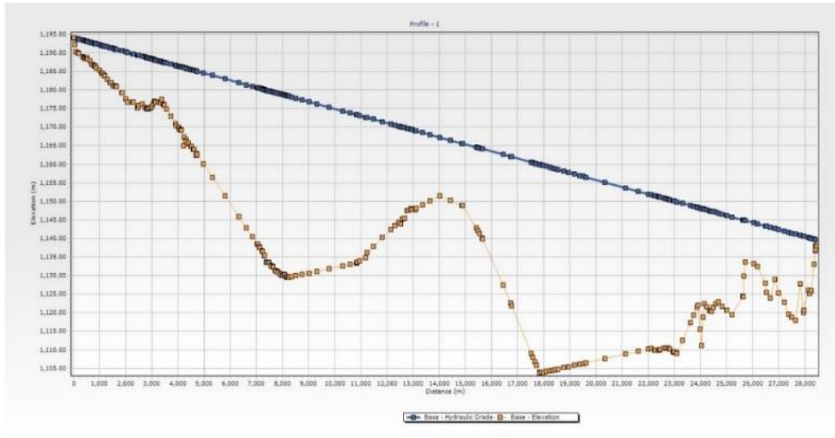
Figure 13. The hydraulic profile of the transmission line in a stable state (from the Kavardah tank to the F zone tank)
