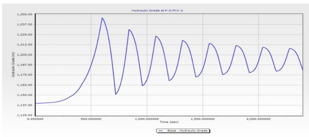
Figure 19. Hydraulic gradient changes, at the end of the route, in case of controlled closing of the valve at the end of the path (from Kavardesh tank to zone F tank).
