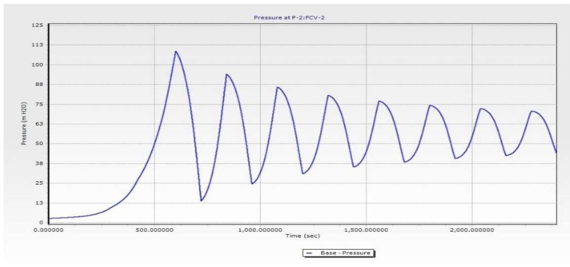
Figure 18. Pressure wave changes at the end of the path in case of controlled closing of the valve at the end of the path (from Kavardesh tank to F zone tank)
