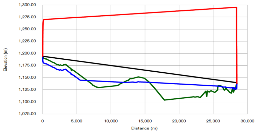
Figure 17. Profile of the minimum and maximum hydraulic gradient, in case of sudden closing of the valve at the end of the path (from Kavardesh tank to F zone tank)
