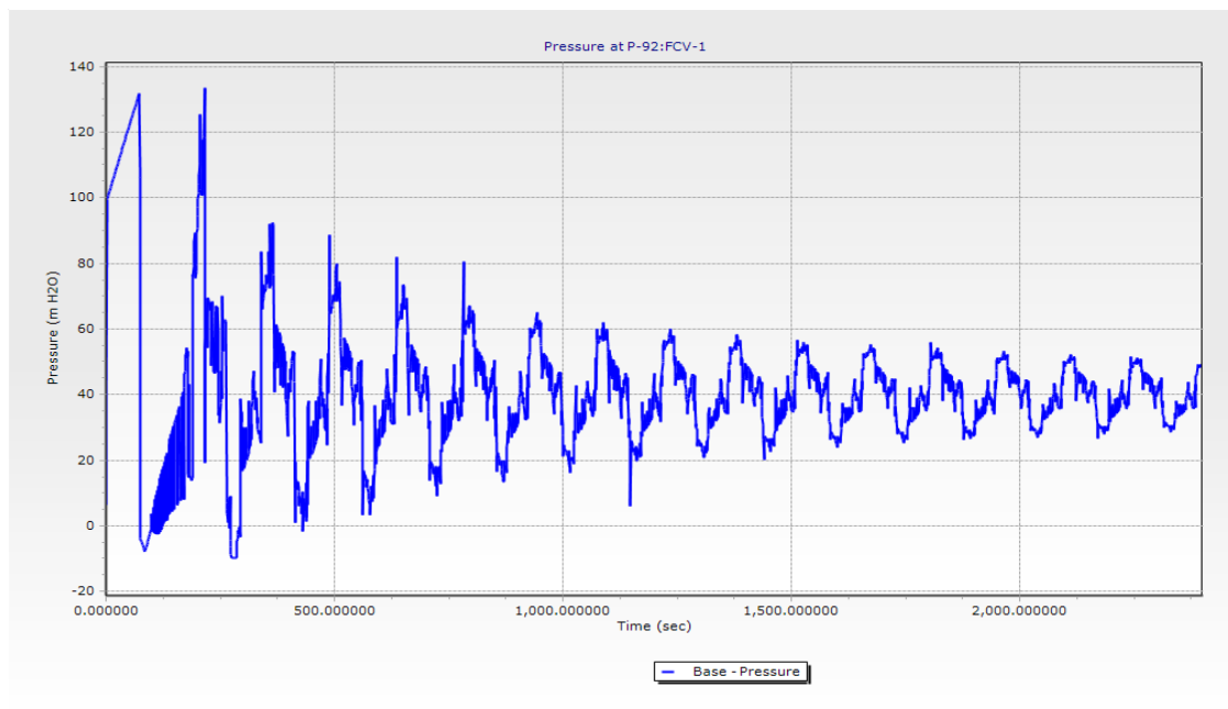
Figure 5. Pressure wave changes at the end of the path in case of sudden closing of the valve at the end of the path (from Islamabad tank to Kavardreh tank)
