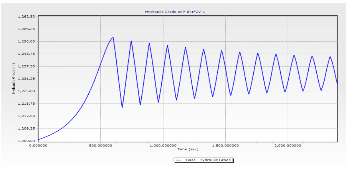
Figure 10. Hydraulic gradient changes at the end of the path in case of controlled closing of the valve at the end of the path (from Islamabad tank to Kavardah tank)
