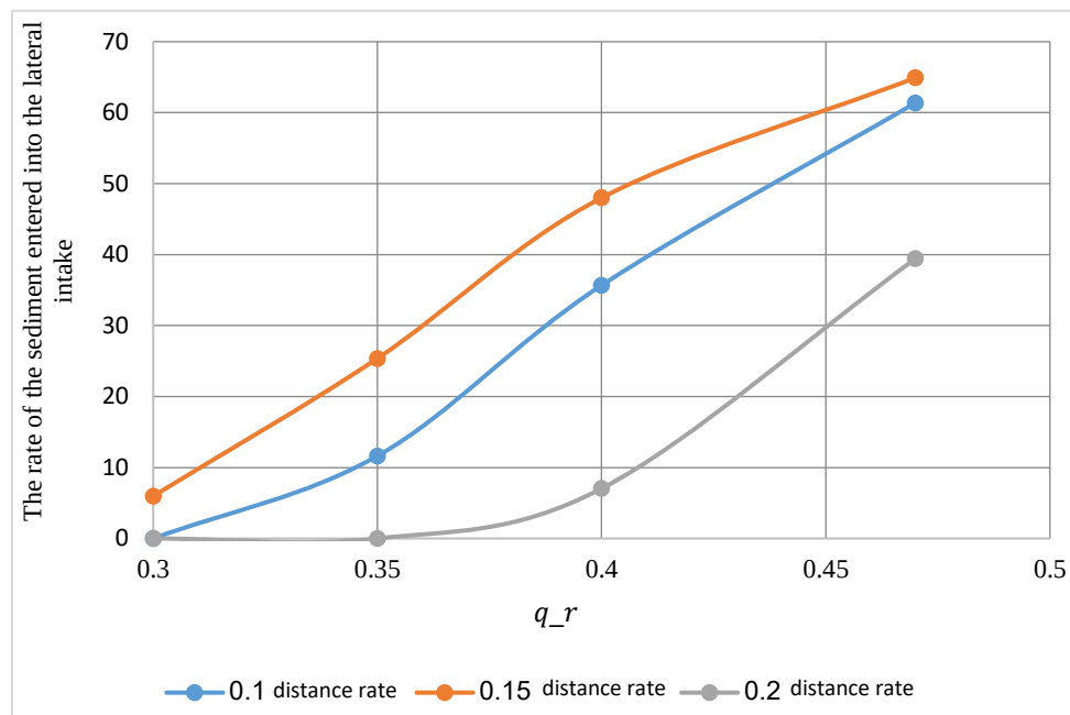
Figure 7. Cumulative diagram for plate angle of 15° based on the variable distance rates.
