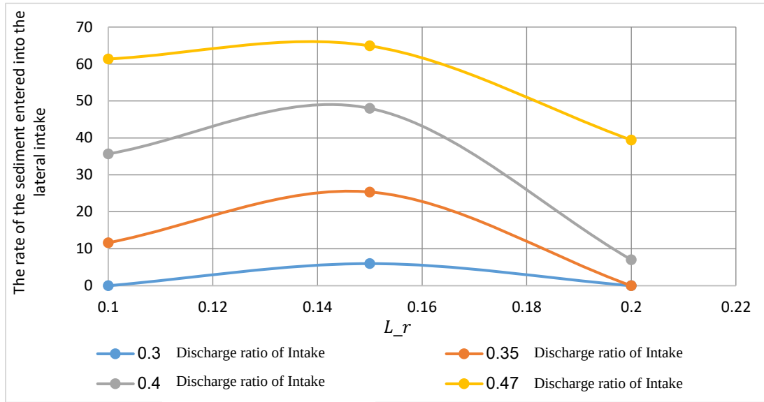
Figure 10. Cumulative diagram for plate angle of 15° and discharge ratio of intake.
