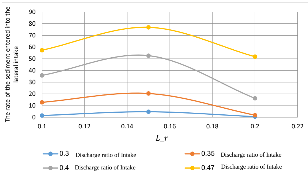
Figure 11. Cumulative diagram for plate angle of 20° and discharge ratio of intake.
