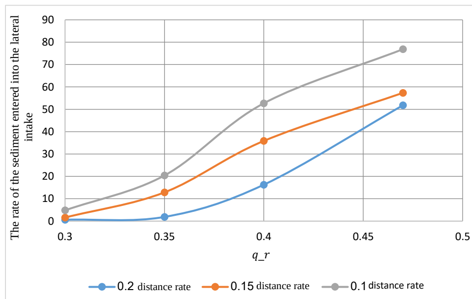
Figure 8. Cumulative diagram for plate angle of 20° based on the variable distance rates.
