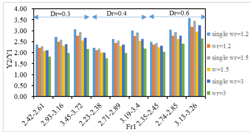
Figure 8. Illustrations of the ratio of (\frac{Y_2}{Y_1}) to the Froude number ( Fr_1 ) for a relative roughness height of 3 compared to a smooth channel.
