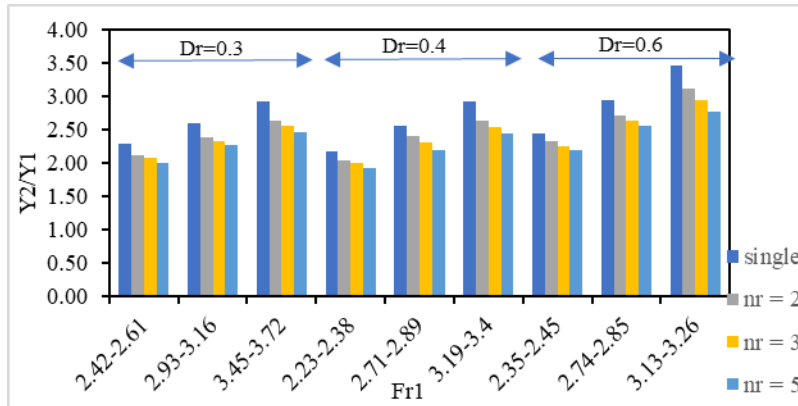
Figure 5. The ratio of ( \frac{Y_2}{Y_1} ) to the Froude number ( Fr_1 ) for a width ratio of 1.5 (with a floodplain width of 22.5 cm) relative to the smooth channel.
