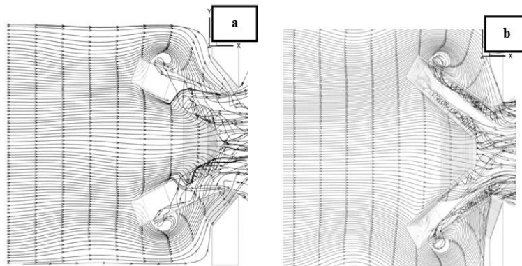
Figure 15. stream lines of the lower layer of the weir a) ATPK45-2 b) ATPK135-2.
