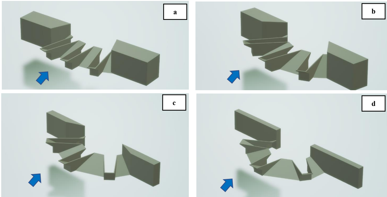
Figure 7. Three-dimensional view ATPKW with three cycles in plan a) 45 degrees b) 90 degrees c) 135 degrees and d) 180 degrees.
