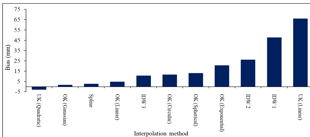
Figure 3. Evaluation of interpolation methods accuracy using BIAS index.
