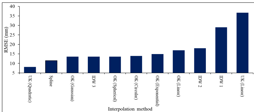
Figure 6. Evaluation of interpolation methods accuracy using RMSE index.
