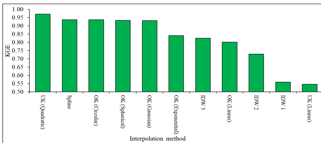
Figure 5. Evaluation of interpolation methods accuracy using KGE index
