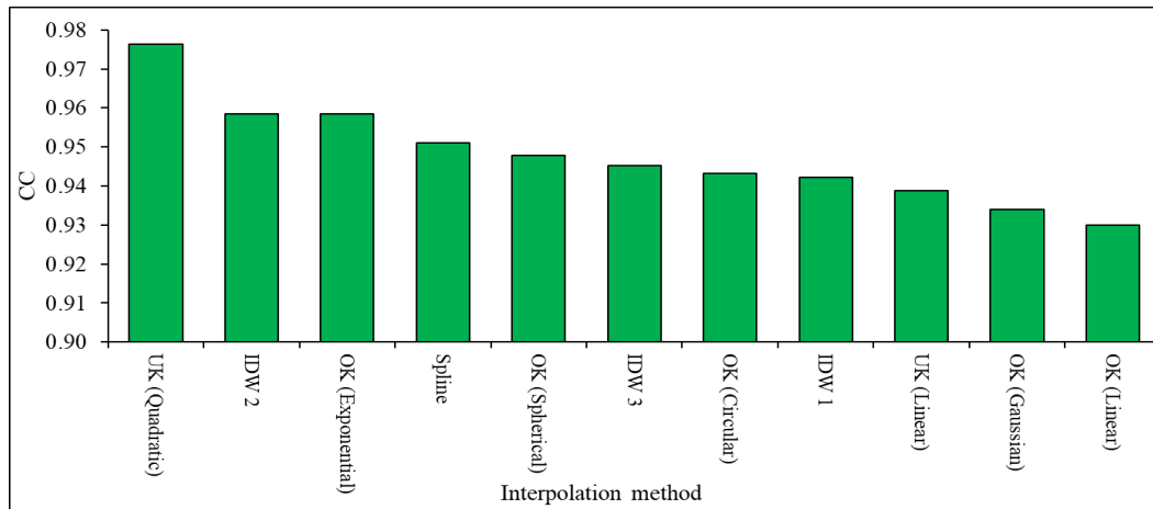
Figure 4. Evaluation of interpolation methods accuracy using CC index.
