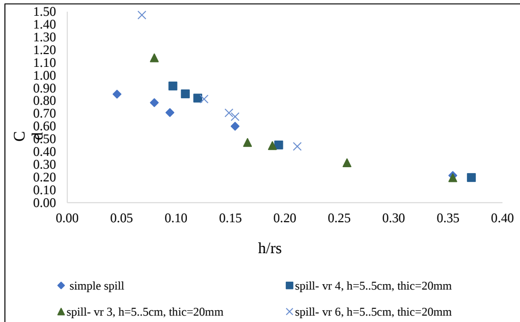
Figure 8. C_d against h/rs (smooth spillway) with low medium v. breaker.
