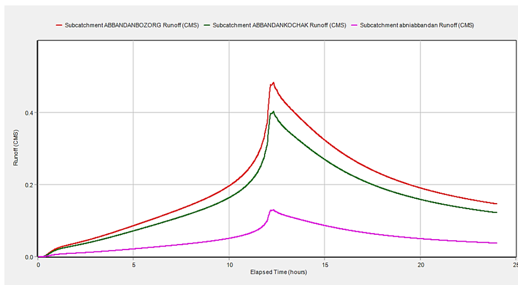
Figure 6. Run-off hydrograph for 3 Abbandans in the 25-year return period.
