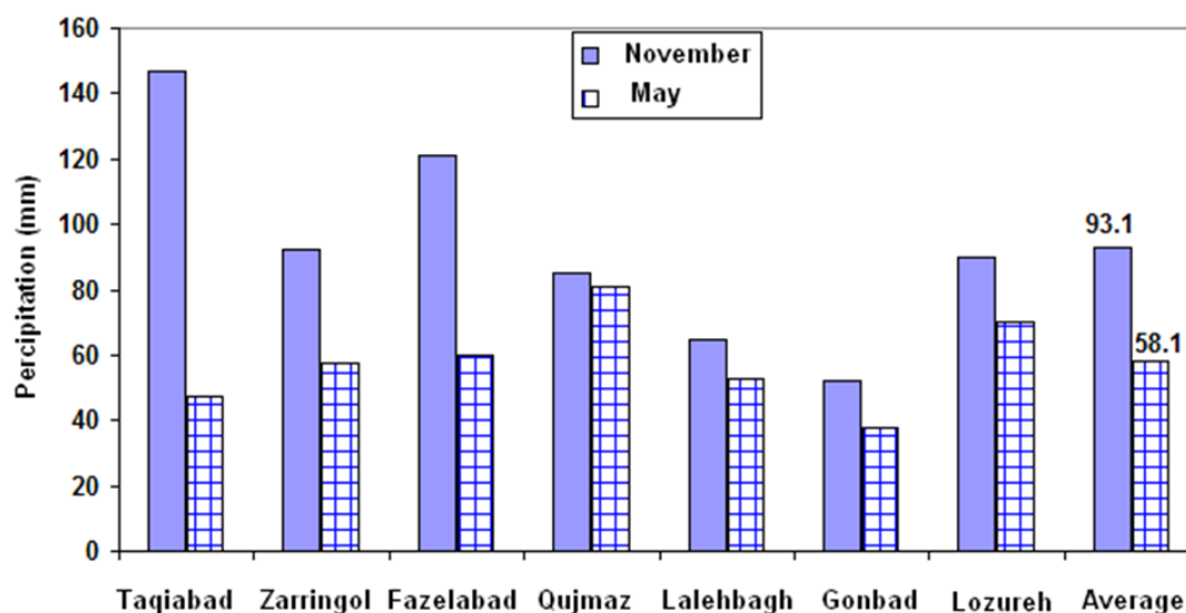
Figure 3. Comparison of precipitation of stations in the region and their average in November 2019 and May 2020.
