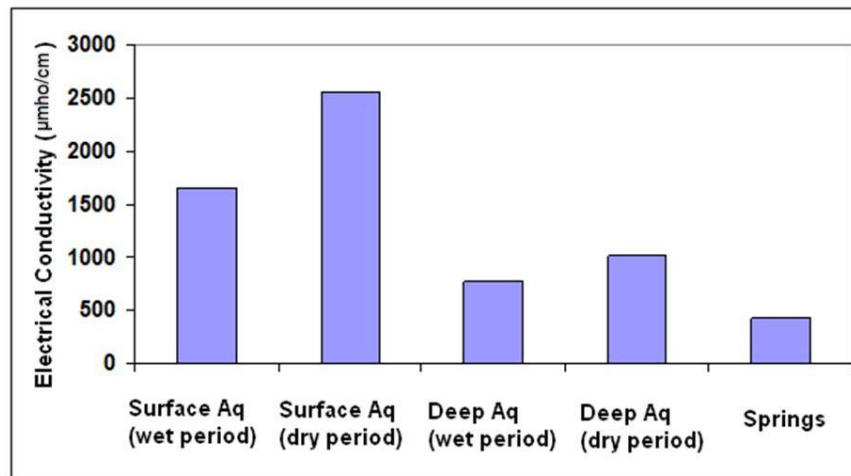
Figure 6. Comparison of the average electrical conductivity in shallow and deep aquifers with springs.
