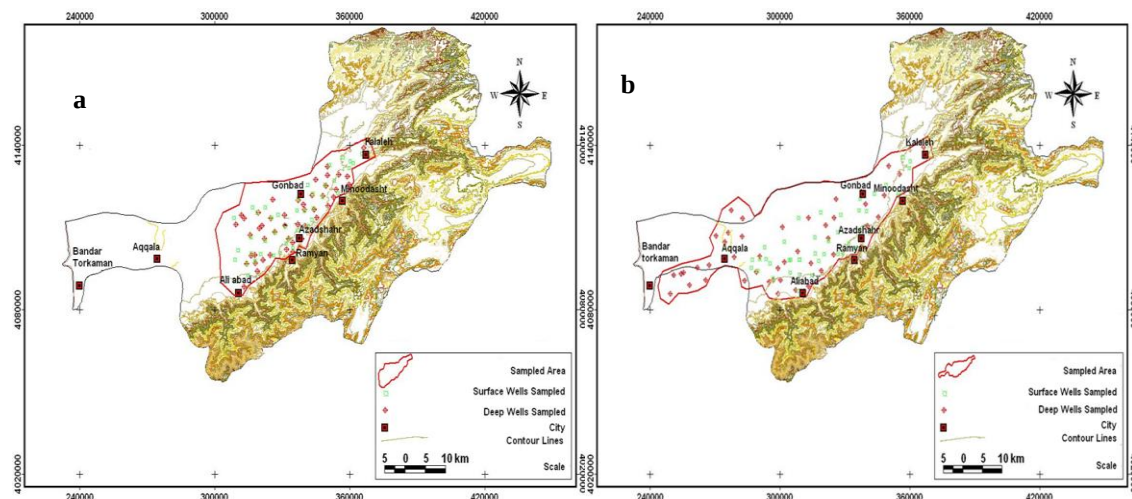
Figure 2. Location of sampling wells in a) November 2019, b) May 2020.
