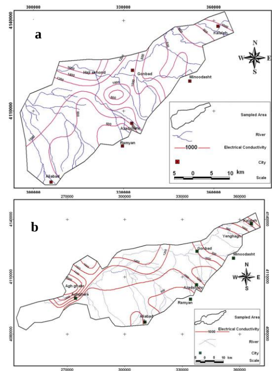
Figure 5. Map of electric conductivity ( \mu\text{mho/cm} ) of deep aquifers in a) November 2019 and b) May 2020.
