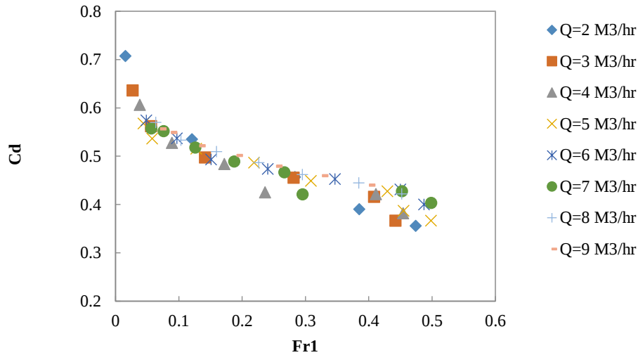
Figure 5. Variations of C_d against Fr_1 in free flow conditions.
